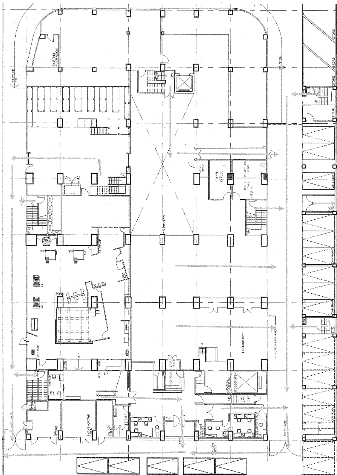
GROUND FLOOR FIRE ESCAPE ROUTE LAYOUT PLAN
